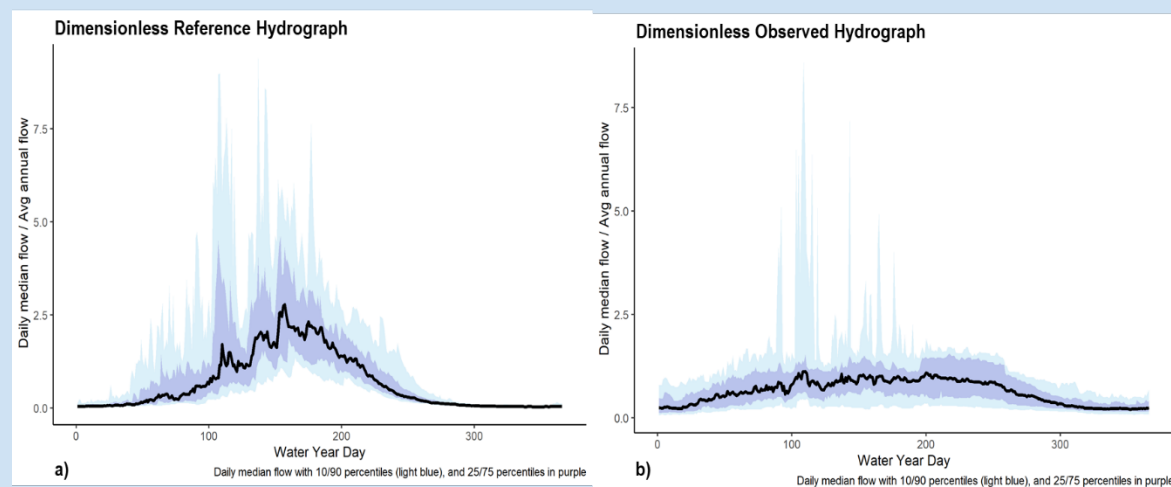
Figure 4.4. An example of a) dimensionless reference hydrograph (DRH) for a low-volume snowmelt and rain stream and b) a dimensionless observed hydrograph for a gage in the Sierra Nevada where flows are altered due to a diversion dam. Both figures were calculated and output from eflows.ucdavis.edu/hydrology .
