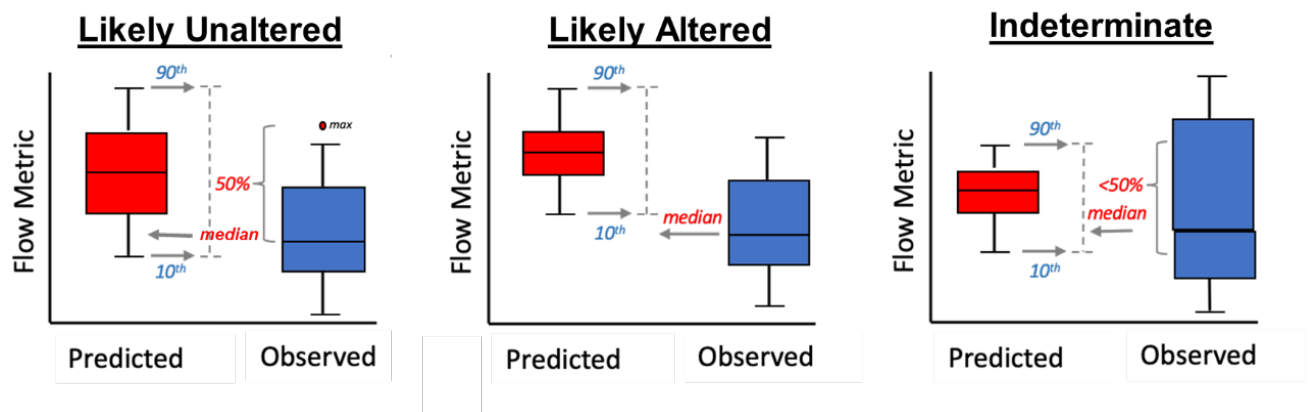
Figure 4.3. Alteration assessment determination for a functional flow metric. Predicted natural ranges for functional flow metrics (in red) represent the ecological flow criteria at a LOI against which observed values (in blue) are compared. The box and whiskers plots represent the range (10 th , 25 th , 50 th , 75 th , and 90 th percentiles) of predicted and observed values for the functional flow metric.
