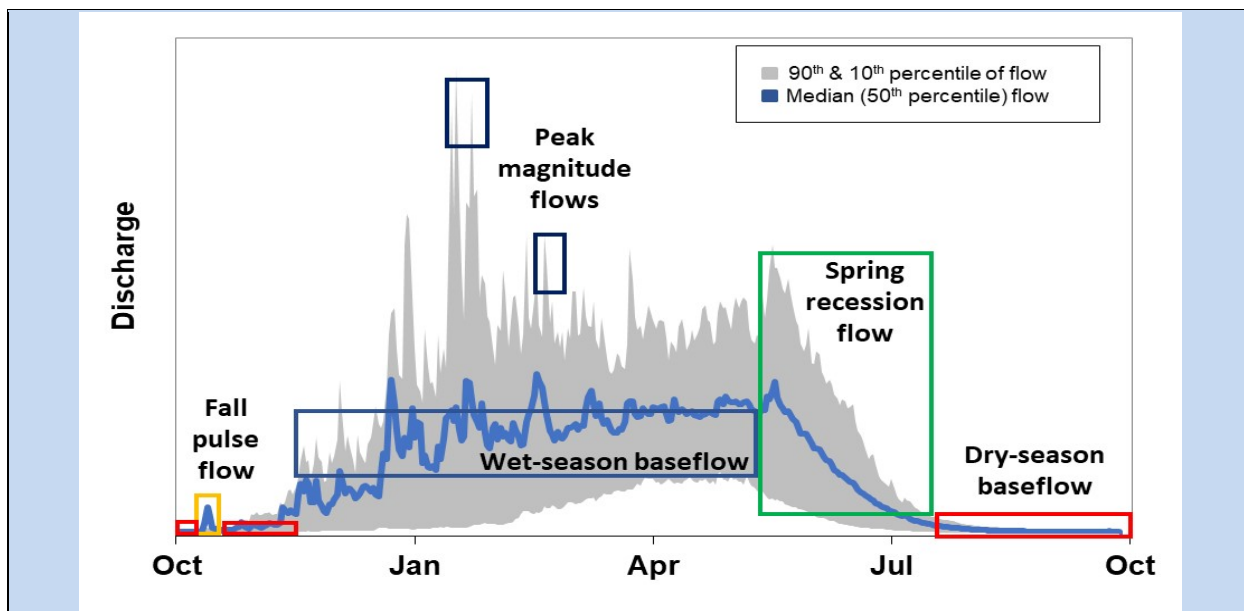
Figure 1.3. Functional flow components for California depicted on a representative hydrograph. Blue line represents median (50 th percentile) daily discharge. Gray shading represents 90 th to 10 th percentiles of daily discharge over the period of record.
