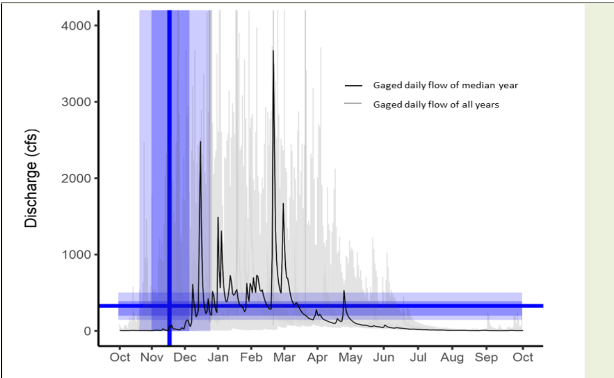
Figure A.2. A hydrograph representing the range of daily flows observed at a flow gage in the study area and the start timing and magnitude of wet season baseflow. The dark line represents the median gauged daily flow, the grey lines are the gauged daily flows for all years. The vertical blue bands show the range of variation (10 th , 25 th , 50 th , 75 th and 90 th percentile) in wet season start timing and the horizontal blue band shows the range of variation (10 th , 25 th , 50 th , 75 th and 90 th percentile) in wet season baseflow magnitude. Source: https://eflows.ucdavis.edu
