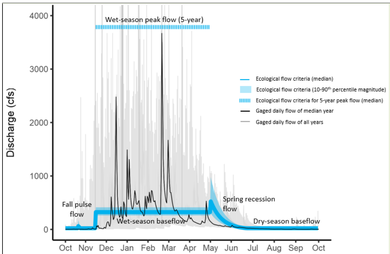
Figure A.6. Ecological flow regime developed from the ecological flow criteria presented in Table A.7. Note that only dry-season baseflow magnitude was determined in Section B, while all other criteria were selected from the natural range of functional flow metrics identified in Section A.
