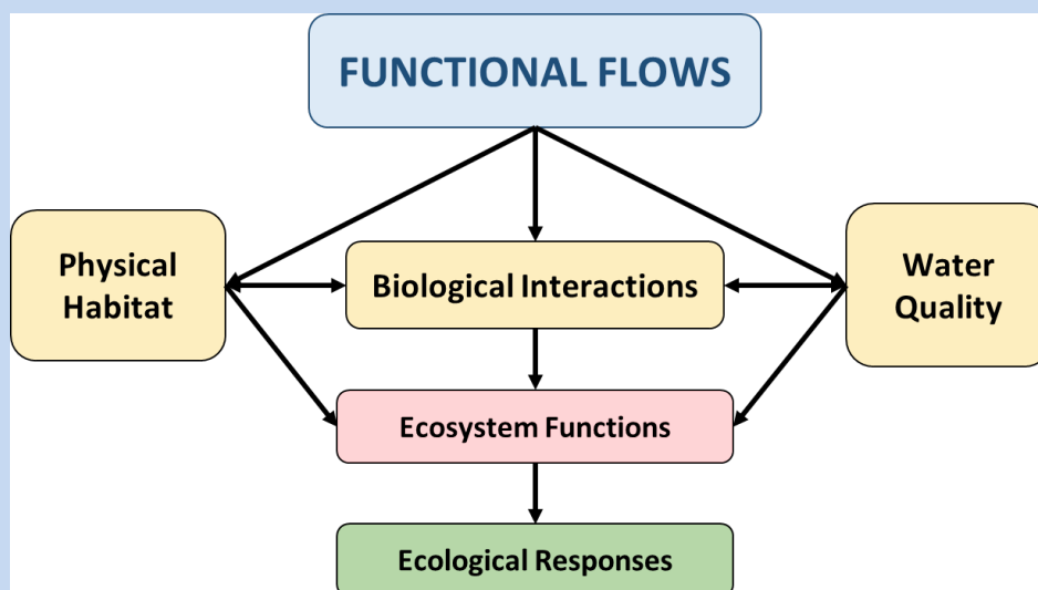
Figure 1.2. Conceptual model demonstrating relationships between functional flows and ecological responses 2 as mediated by factors such as physical habitat, water quality, and biological interactions. Together, these interacting relationships support ecosystem functions that control ecological responses and sustain healthy river and stream ecosystems. Adapted from Poff et al. 1997.
