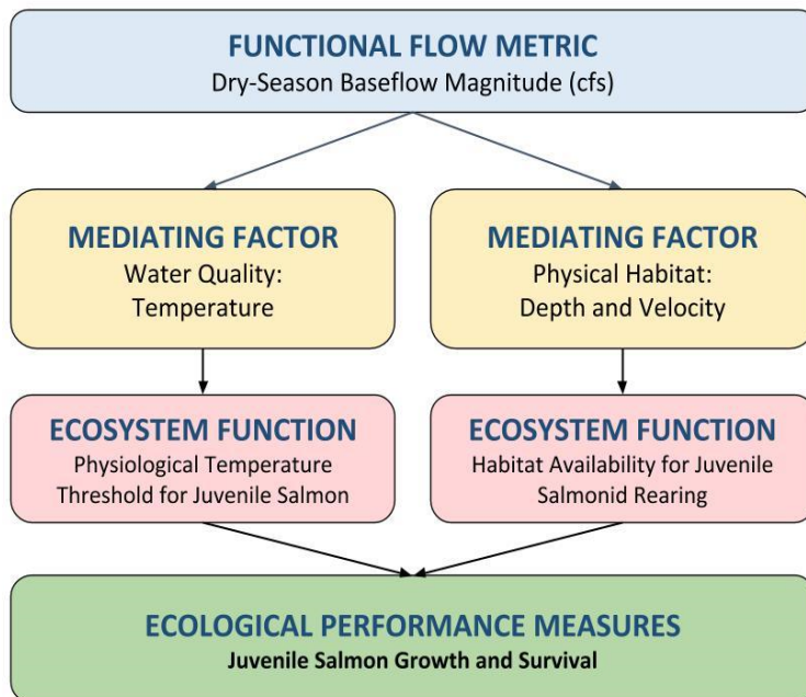
Figure A.4. Conceptual model linking the focal flow component in a coastal watershed in Northern California (dry-season baseflow) with mediating factors, ecosystem functions (as defined in table A.3), and ecological performance measures that relate to the ecological management goal of healthy salmon populations.
