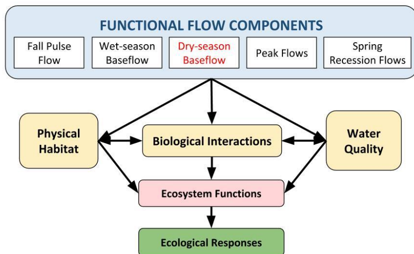
Figure 3.2. Generic conceptual model demonstrating relationships between a functional flow component, ecosystem functions, and ecological response as mediated by factors such as physical habitat, water quality, and biological interactions. This figure can be used as a starting point when developing conceptual models for focal functional flow components in Step 6. Adapted from Poff et al. 1997.
